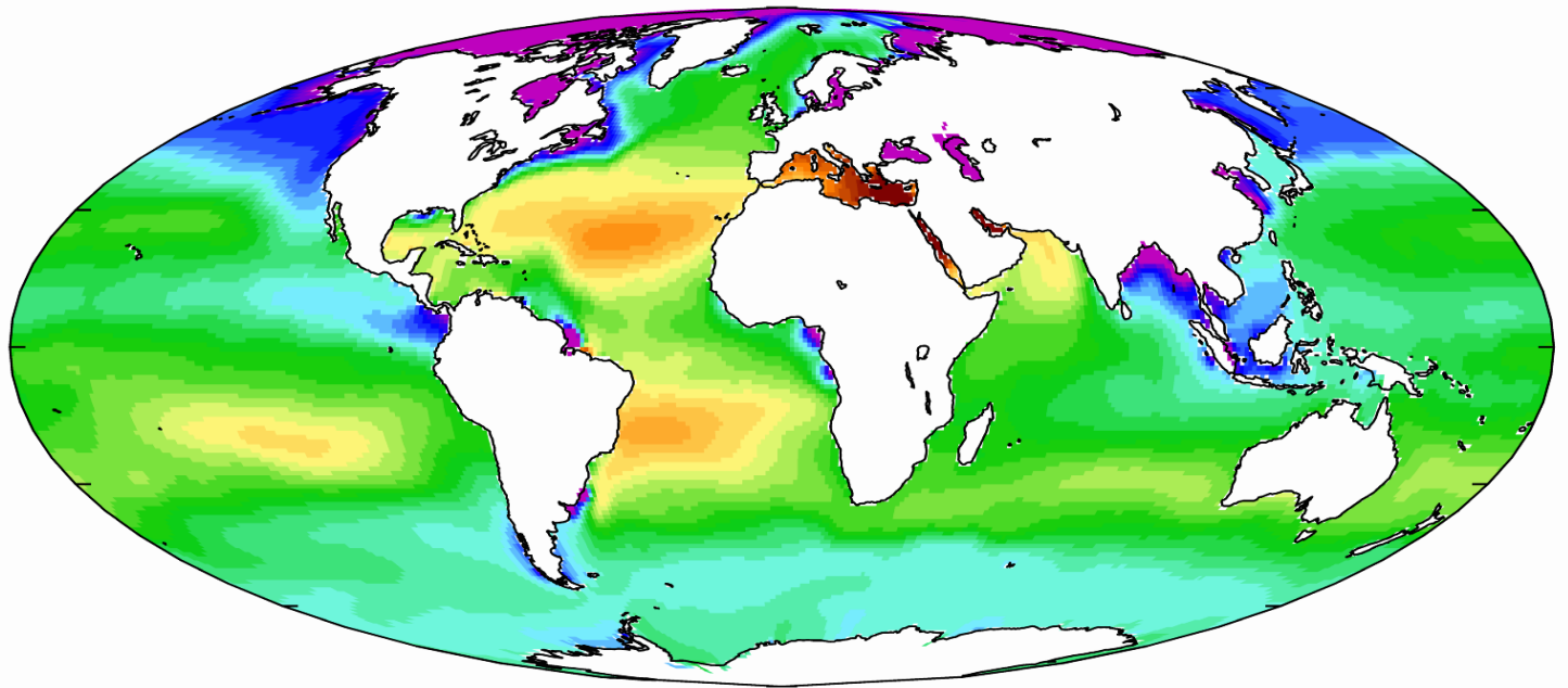
Sea-surface salinity [PSU]
